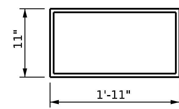
E5 (REQ'D) PLAN VIEW OF ELASTOMERIC BEARING
